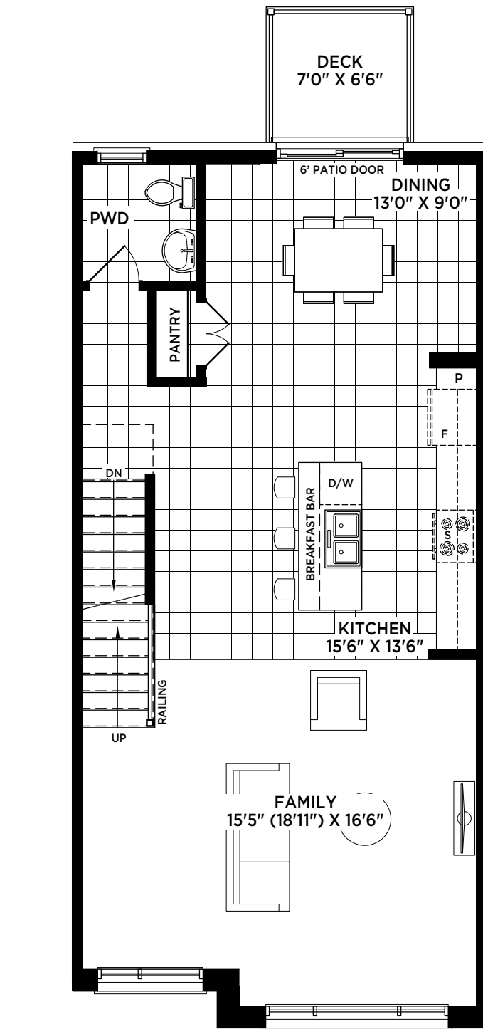
MAIN FLOOR
